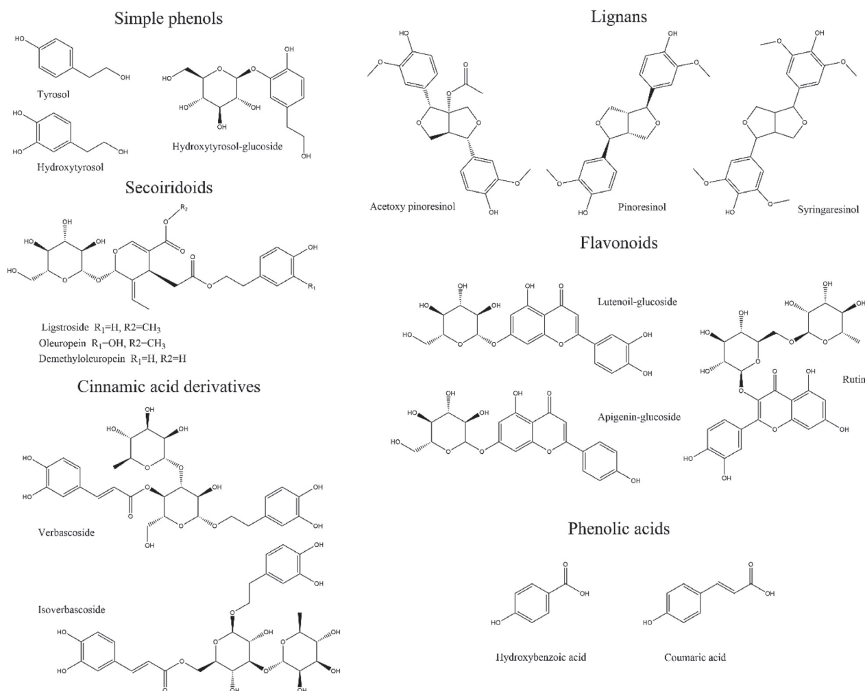
Fig. 1. Phenolic classes and structures of main phenolic compounds in olive leaves [4]
