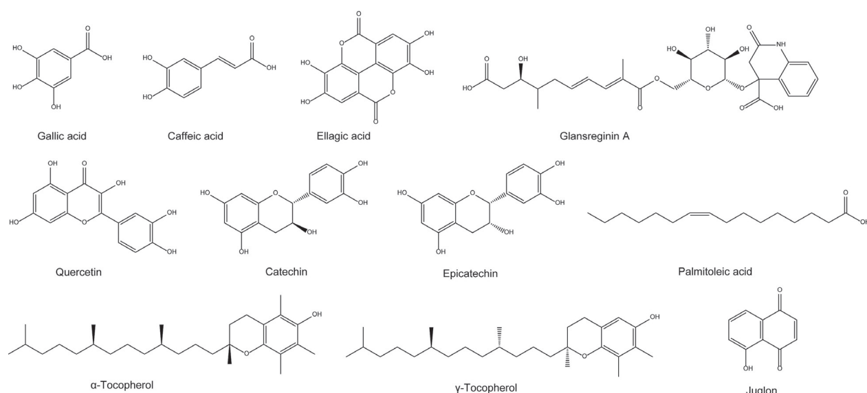
Fig. 3. Structural representation of selected phytochemicals reported in walnut-derived materials, including phenolic and non-phenolic bioactive compounds. adapted from [10]
