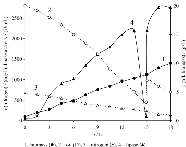
Fig. 1. The time course of exponential growth of Y. lipolytica 704 on rapeseed oil.
