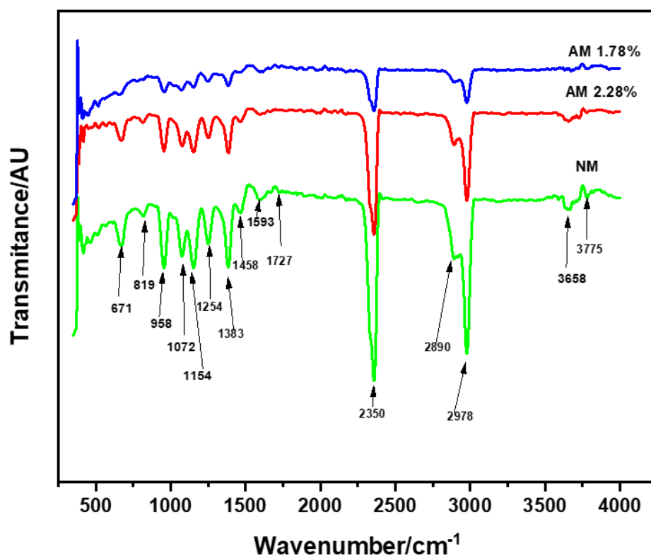
Fig. 1. Spectra of native mucilage (NM) and mucilage acetylated to 1.78 % (AM 1.78 %) and mucilage acetylated to 2.28 % (AM 2.28 %) of Opuntia atropes obtained by Fourier Transform Infrared Spectroscopy (FTIR)
