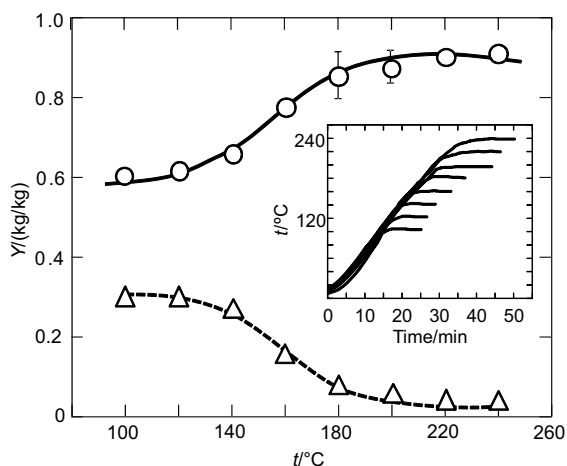
Fig. 2. Yields of the liquid extracts (O) and solid residues (Δ) obtained after subcritical water treatment of raw krill at various temperatures. Inset: temperature profiles during the treatments
